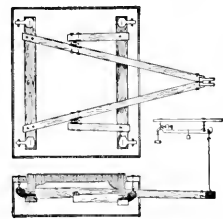
- Patent of 1831 -
